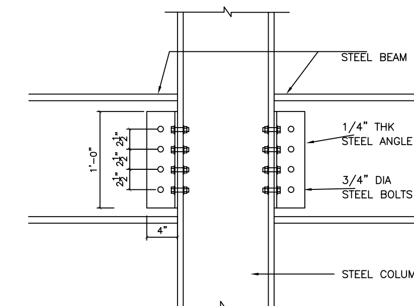
33K CONNECTION
