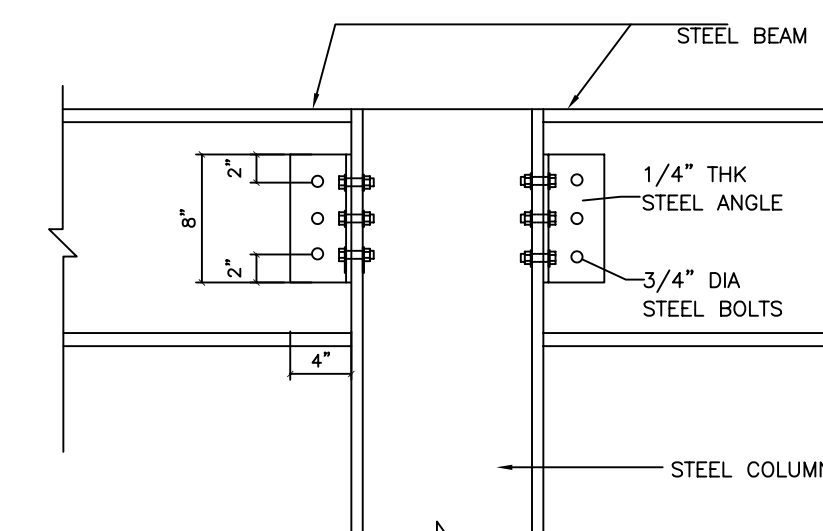
12K CONNECTION
