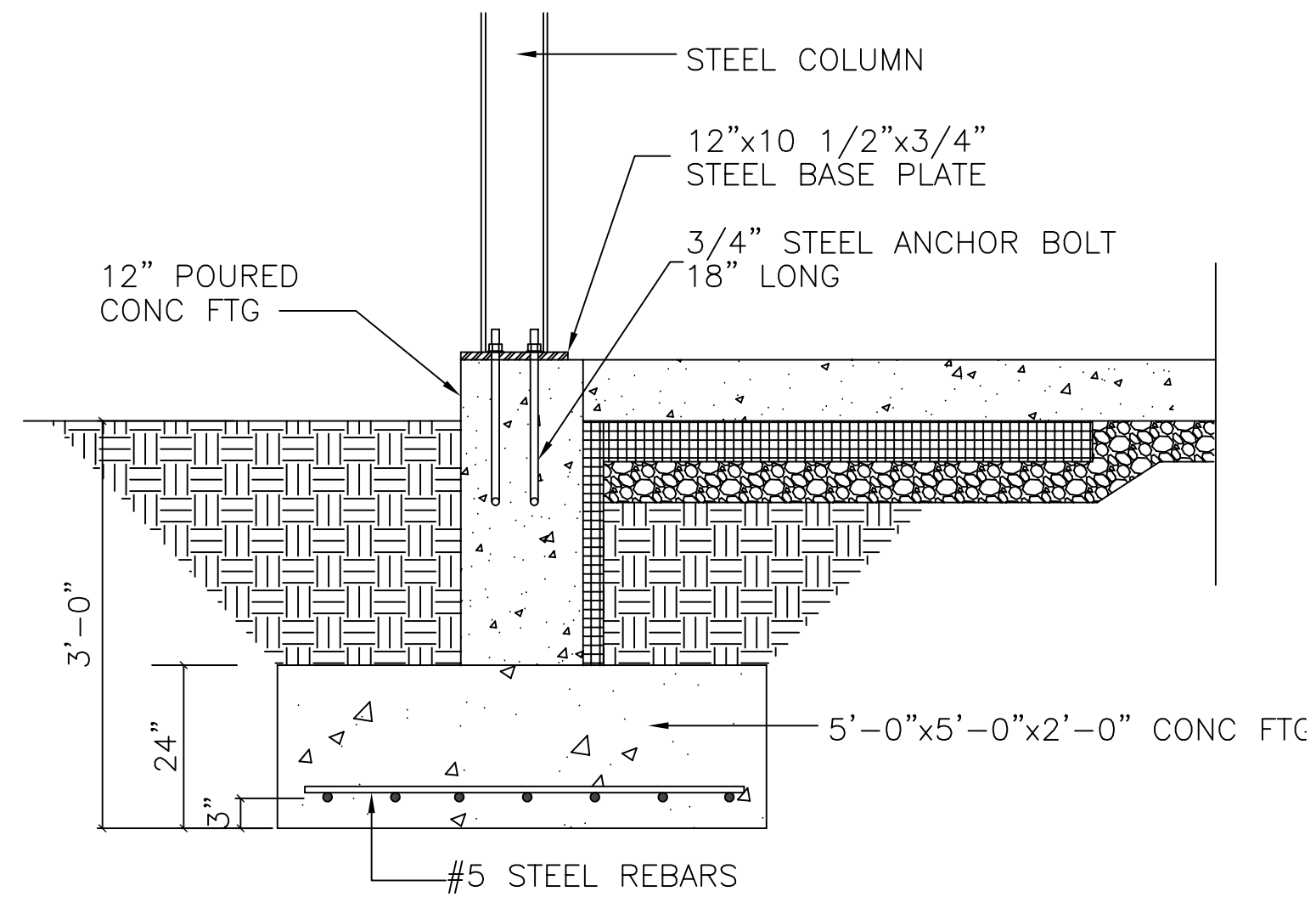
FOUNDATION WALL DETAIL @ COLUMN SCALE: 3/4"=1'-0"
