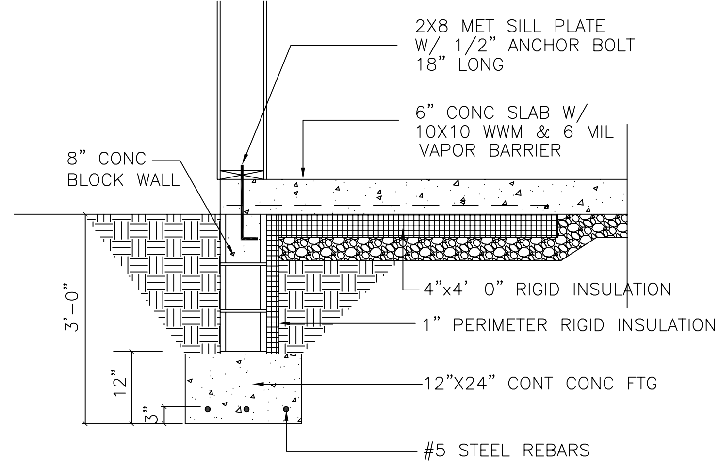
FOUNDATION WALL DETAIL SCALE: 3/4"=1'-0"
