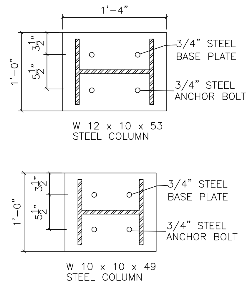
COLUMN BASE PLATE DETAILS SCALE: NTS
