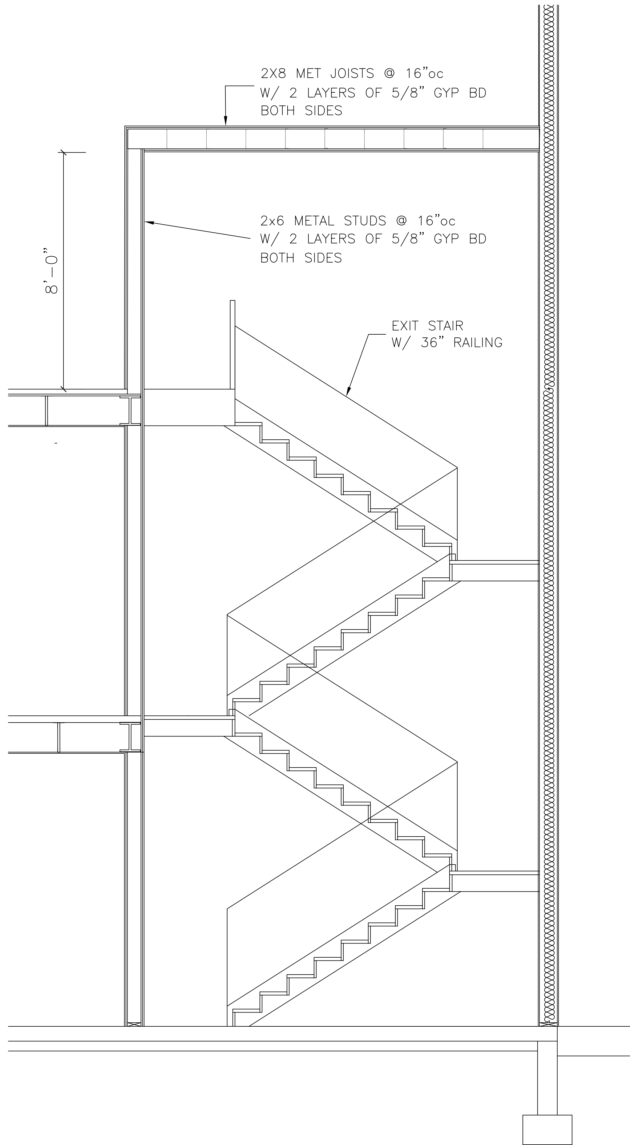
SECTION @ INTERIOR EXIT STAIR SCALE: 3/8"=1'-0"
