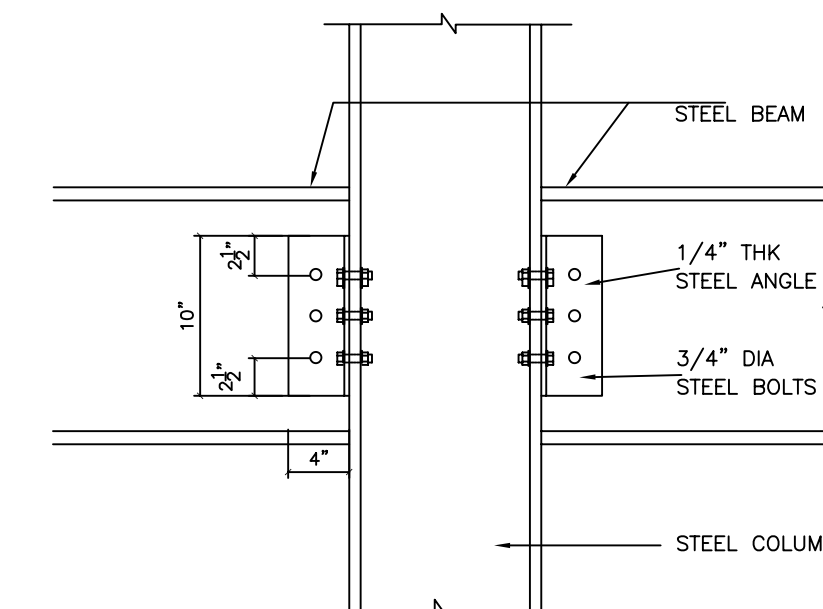
22K CONNECTION
