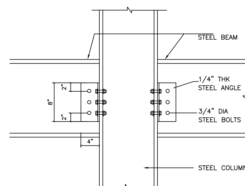
15K CONNECTION
