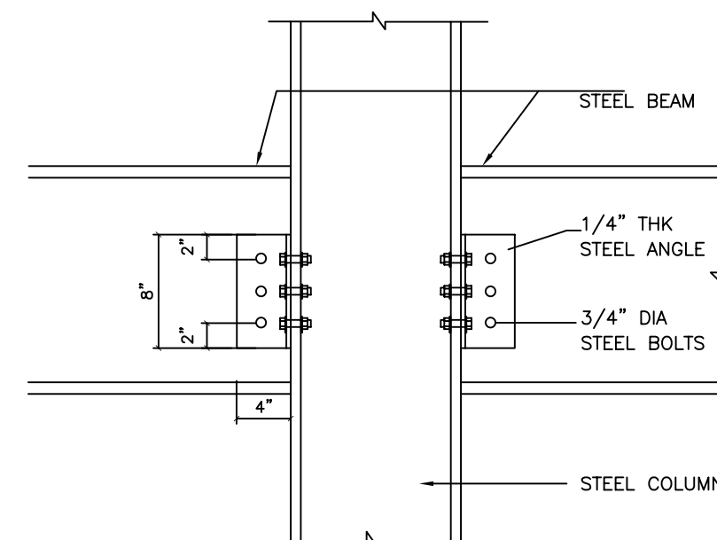
17K CONNECTION
