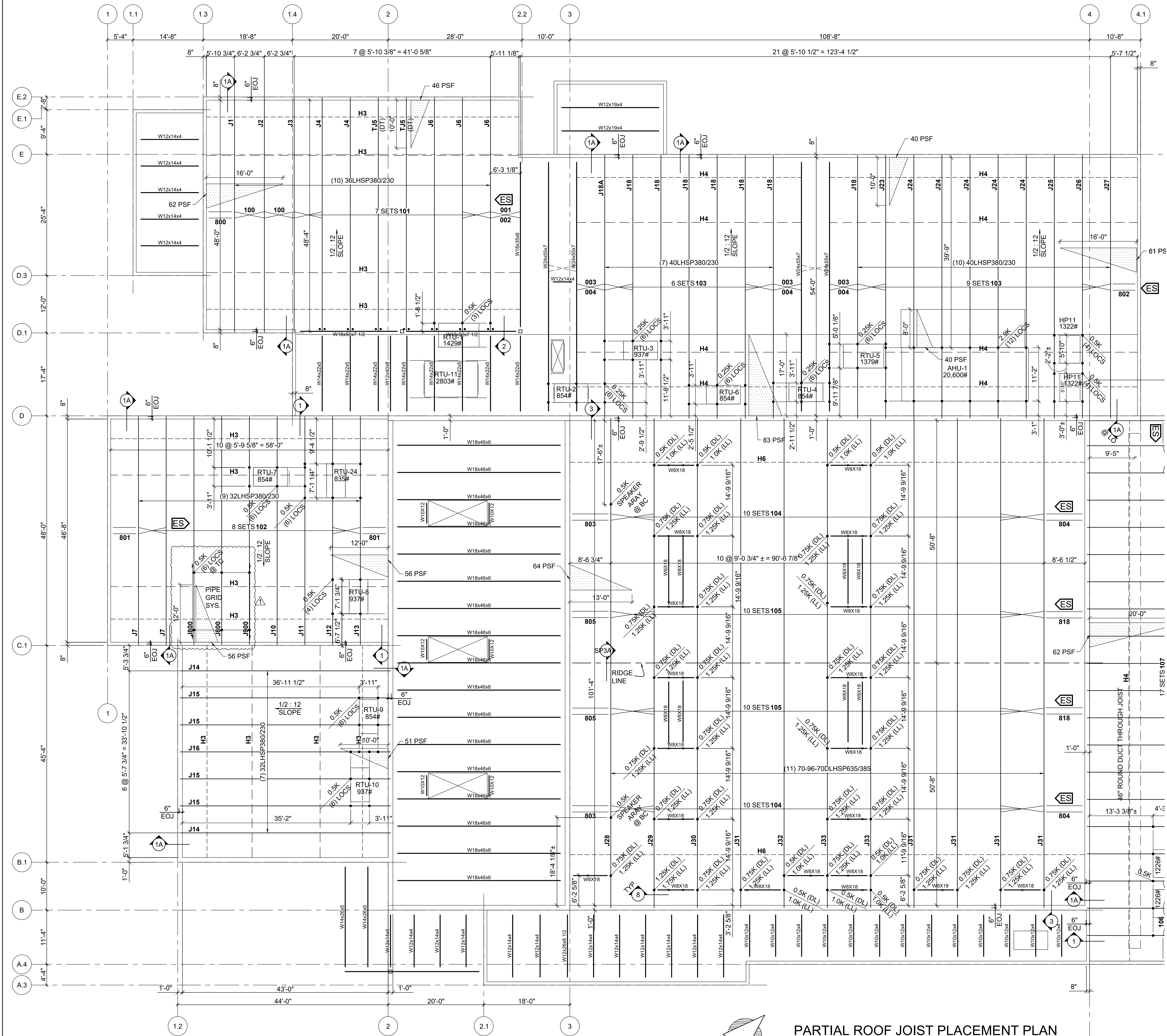
PARTIAL ROOF JOIST PLACEMENT PLAN [SEQ. 5 & SEQ. 4 (SPliced JOISTS)] [REF.: S131]
